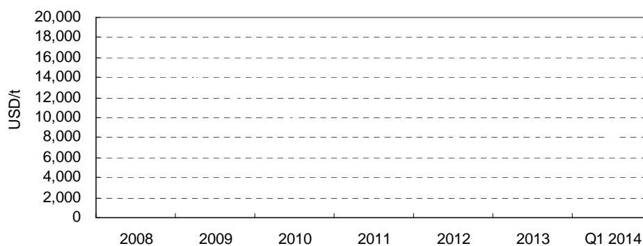
Figure 3.2-1 Annual ex-work price of 2,6-dimethyl aniline in China, 2008-Q1 2014
